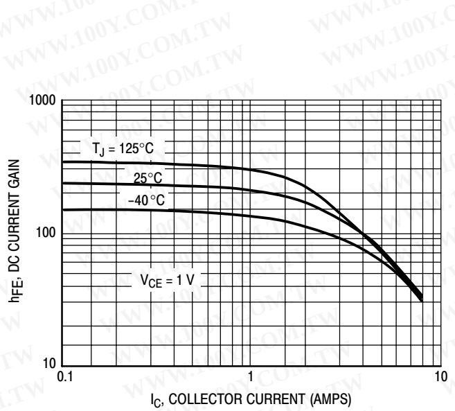
Figure 7. MJD45H11 Current Gain versus Temperature
